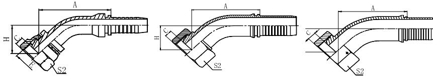
45° BSP FEMALE MULTISEAL
