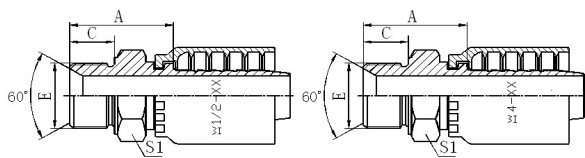
METRIC MALE DOUBLE USE FOR 60° CONE SEAT OR BONDED SEAL
