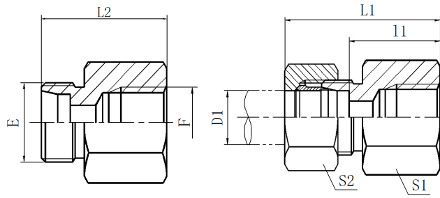
METRIC MALE 24° CONE/METRIC FEMALE STUD FITTINGS
