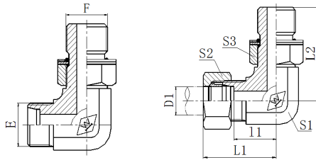
90° ELBOW METRIC MALE 24° CONE / BSP ADJUSTABLE ORING SEAL
