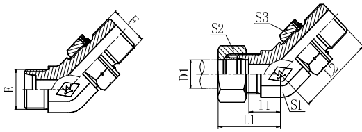
45° ELBOW METRIC MALE 24° CONE / BSP ADJUSTABLE ORING SEAL
